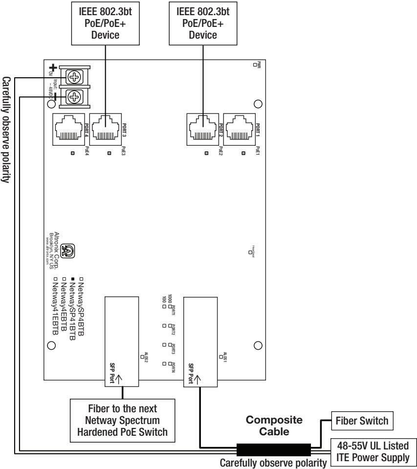
Fig. 2 - NetWaySP41BTB/NetWaySP41BTWPN – Typical Application with Composite Cable
