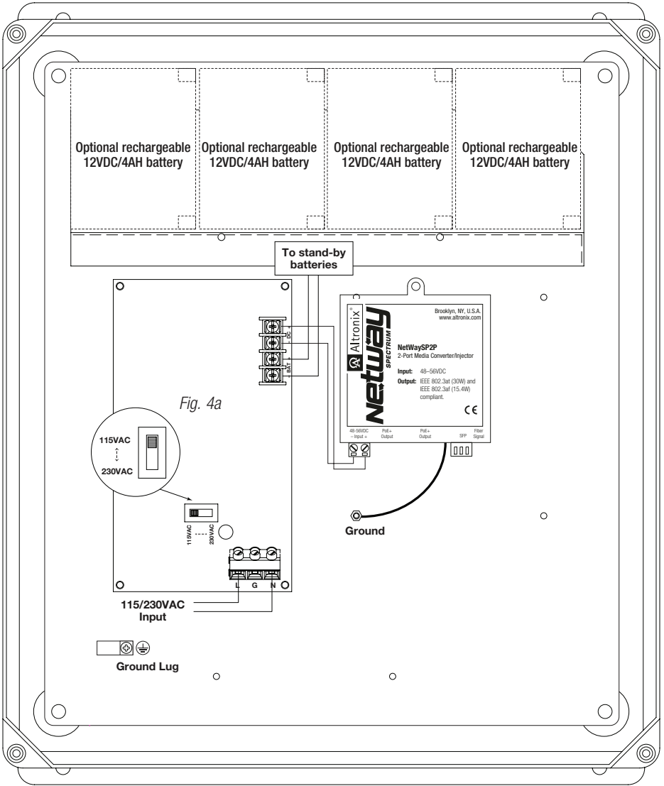
Fig. 4 - NetWaySP2PWPX Configuration
