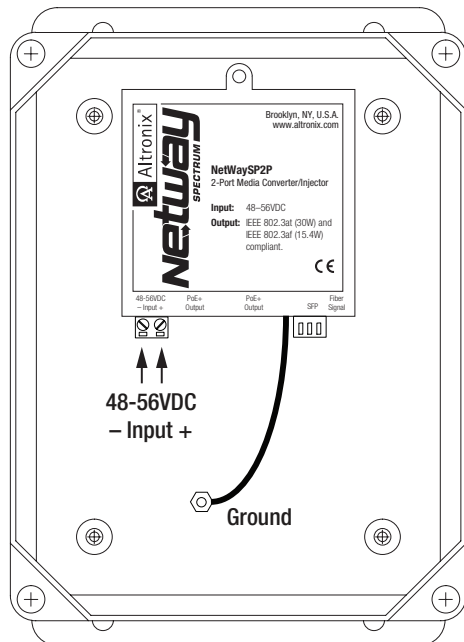
Fig. 2 - NetWaySP2PWPW Configuration
